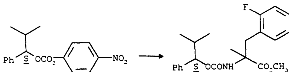
Isomer II
