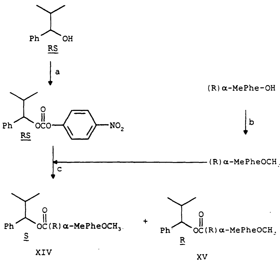
SCHEME 9
