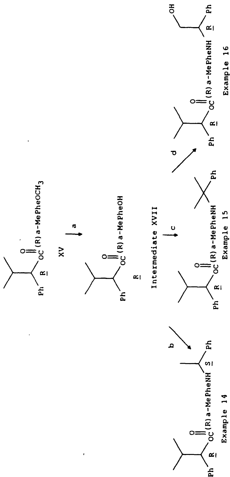
SCHEME 11
