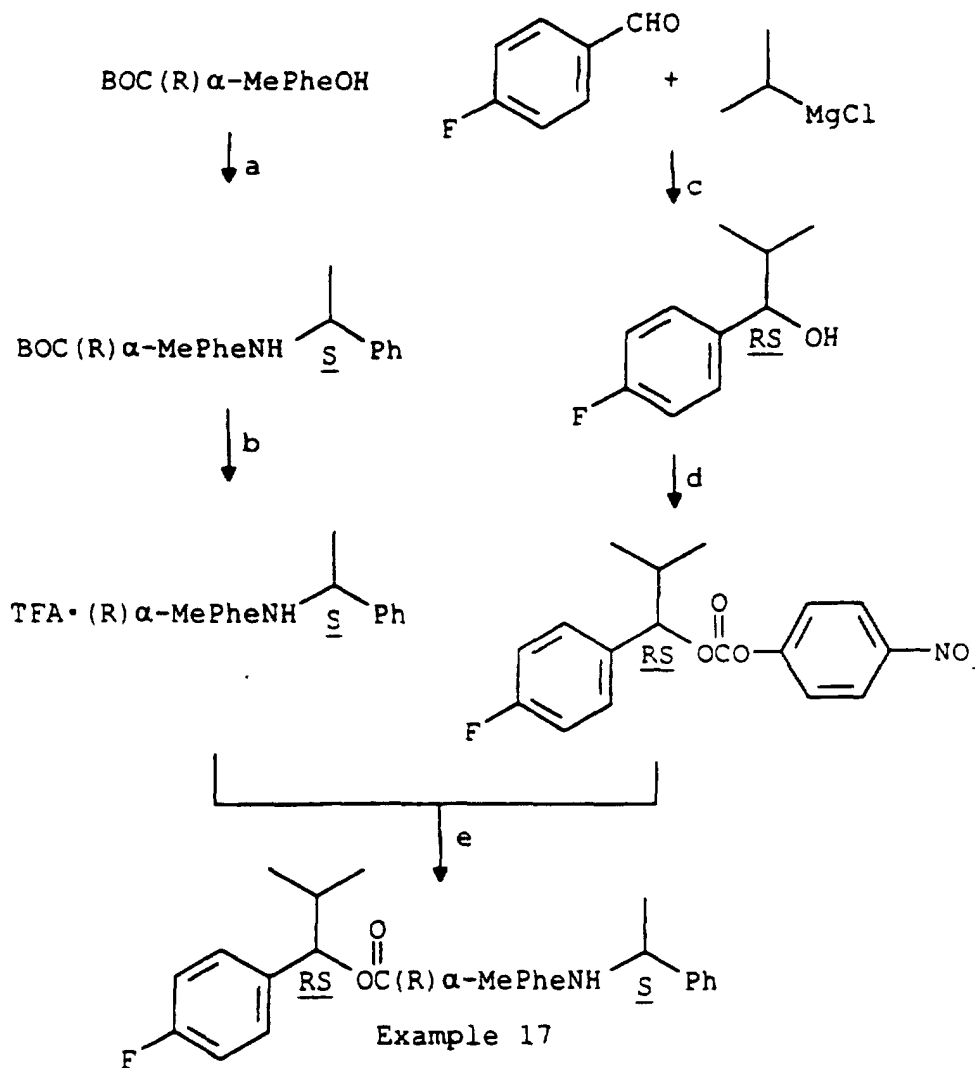
SCHEME 12
