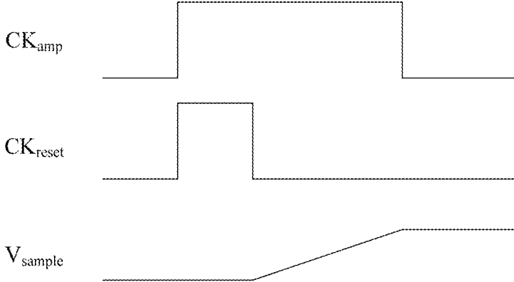
Voltage timing diagram
