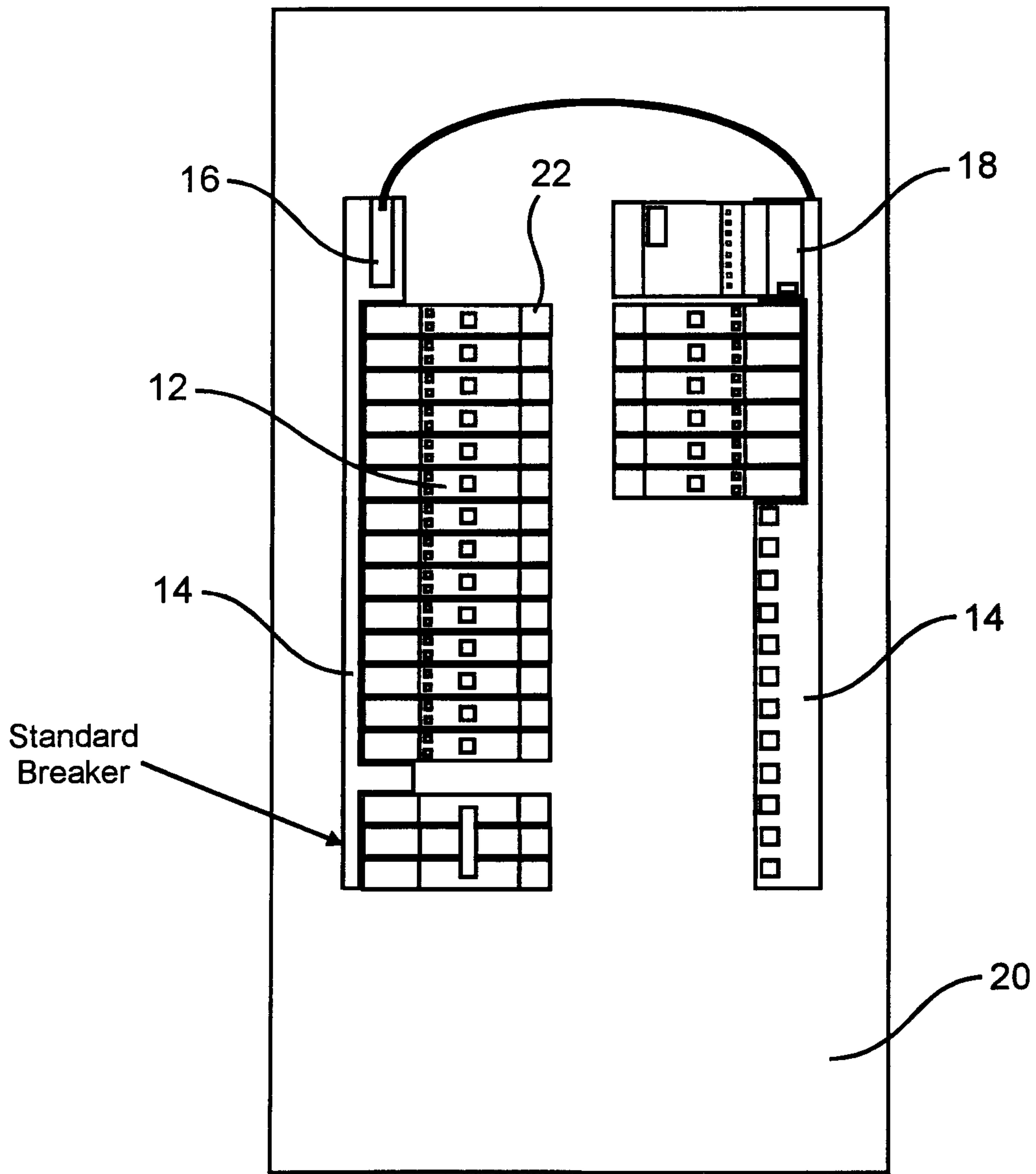
Base System Gem3 Components
