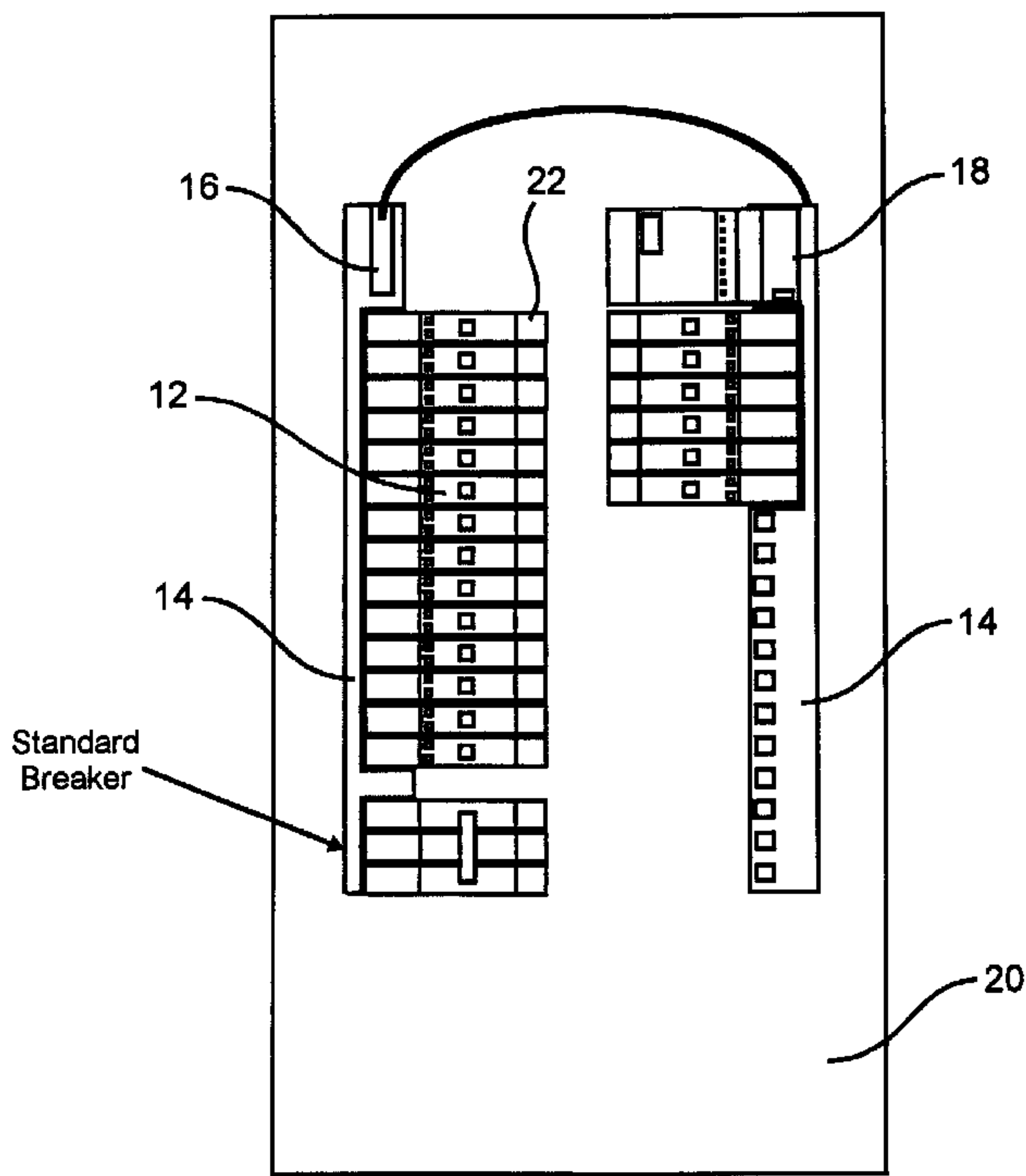
Base System Gem3 Components
