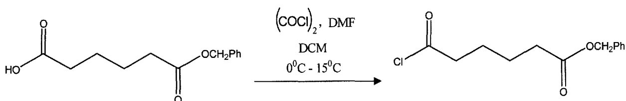
Scheme 6
