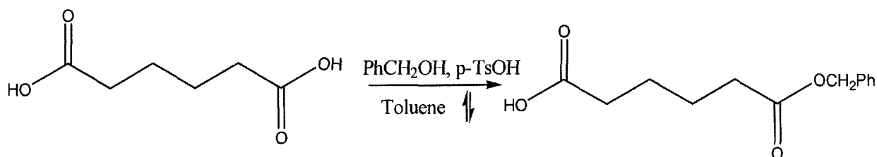
Scheme 5
