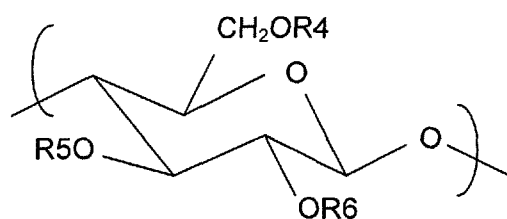
Formula II
