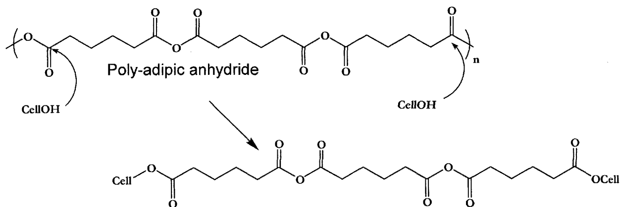
Scheme 7 (CellOH=cellulose)
