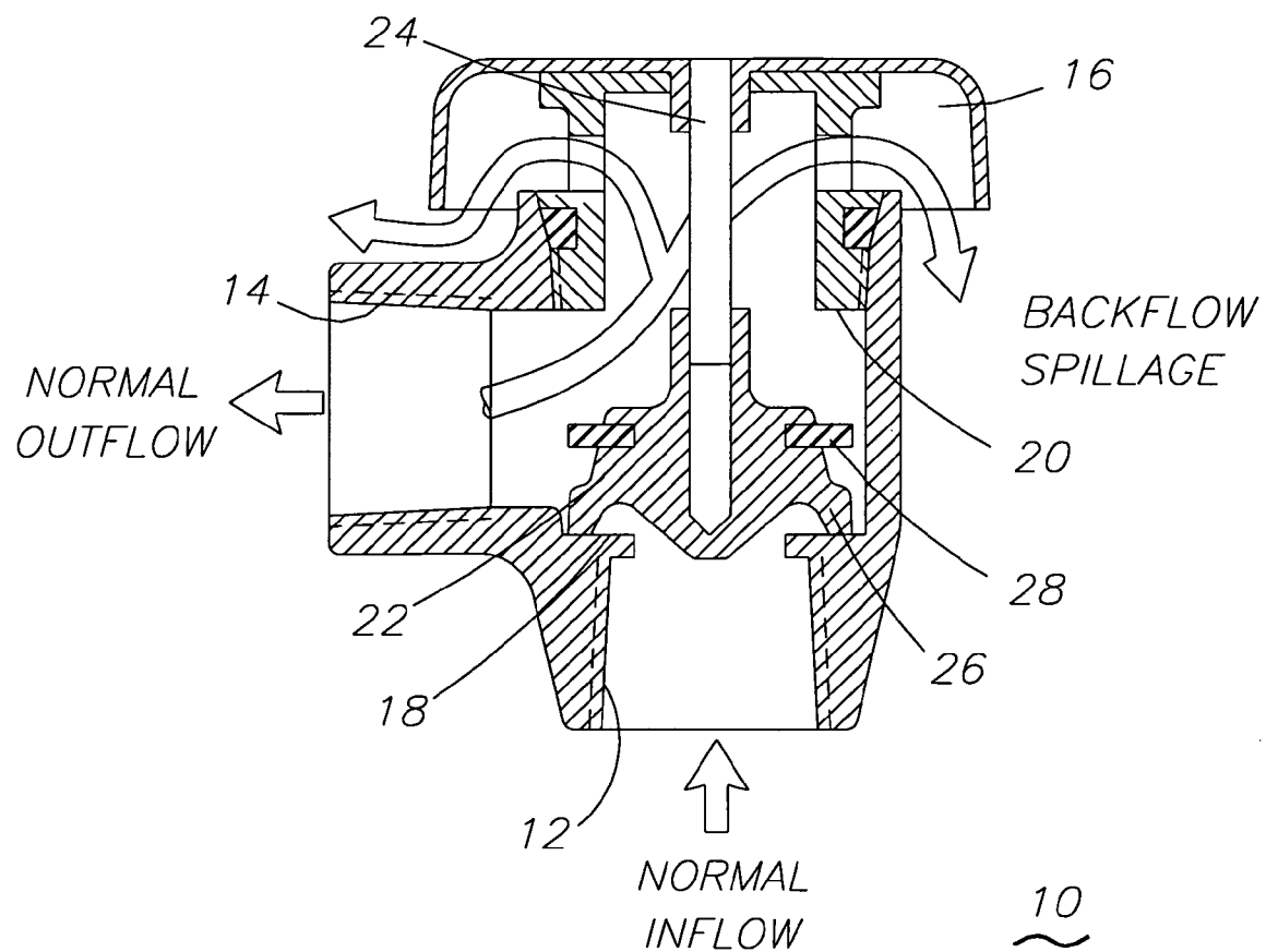
FIG. 1 (PRIOR ART)
