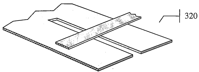
(c) Microstrip crossing over a slotline
