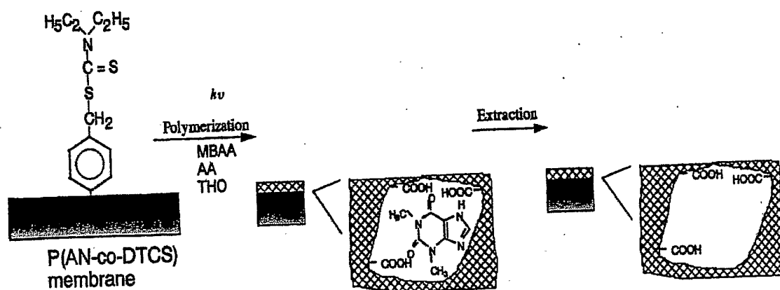
FIG. 3 SURFACE IMPRINTING WITH PHOTOOXIDATION (KOBAYASHI ET AL, 1997)
