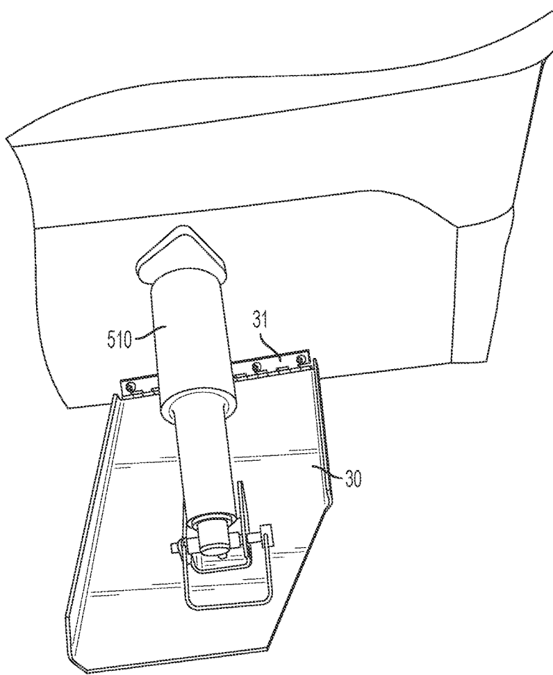
FIG. 2 PRIOR ART
