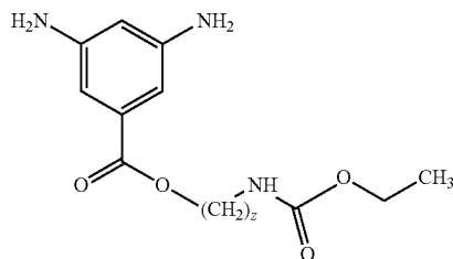
Structure of Diamine 1 (z = 2) [(Ethoxycarbonyl)amino]ethyl 3,5-diaminobenzoate
