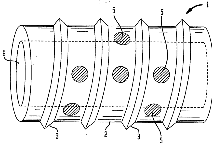
FIG. 14 (PRIOR ART)
