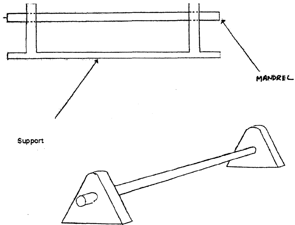
FIG. 3 Wedge Bend Test Piece and Apparatus.
