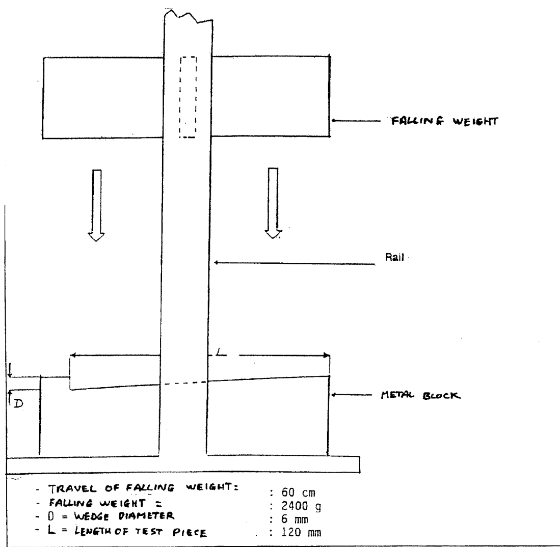
FIG. 4 Diagram of Bending Apparatus
