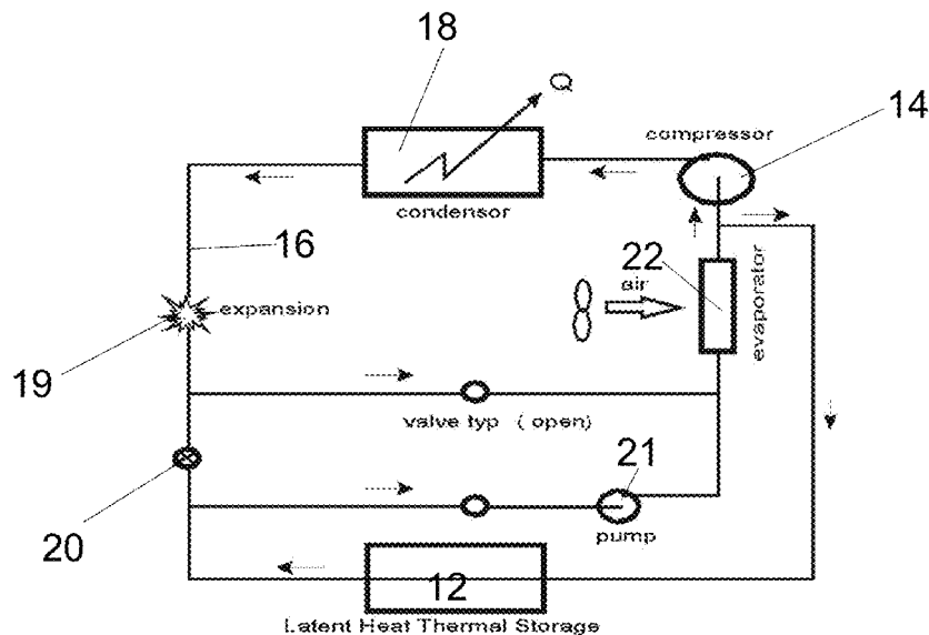
Direct Expansion & Thermal Storage - day operation & night A/C
