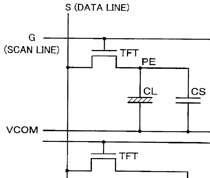
FIG. 12A STORAGE CAPACITANCE METHOD
