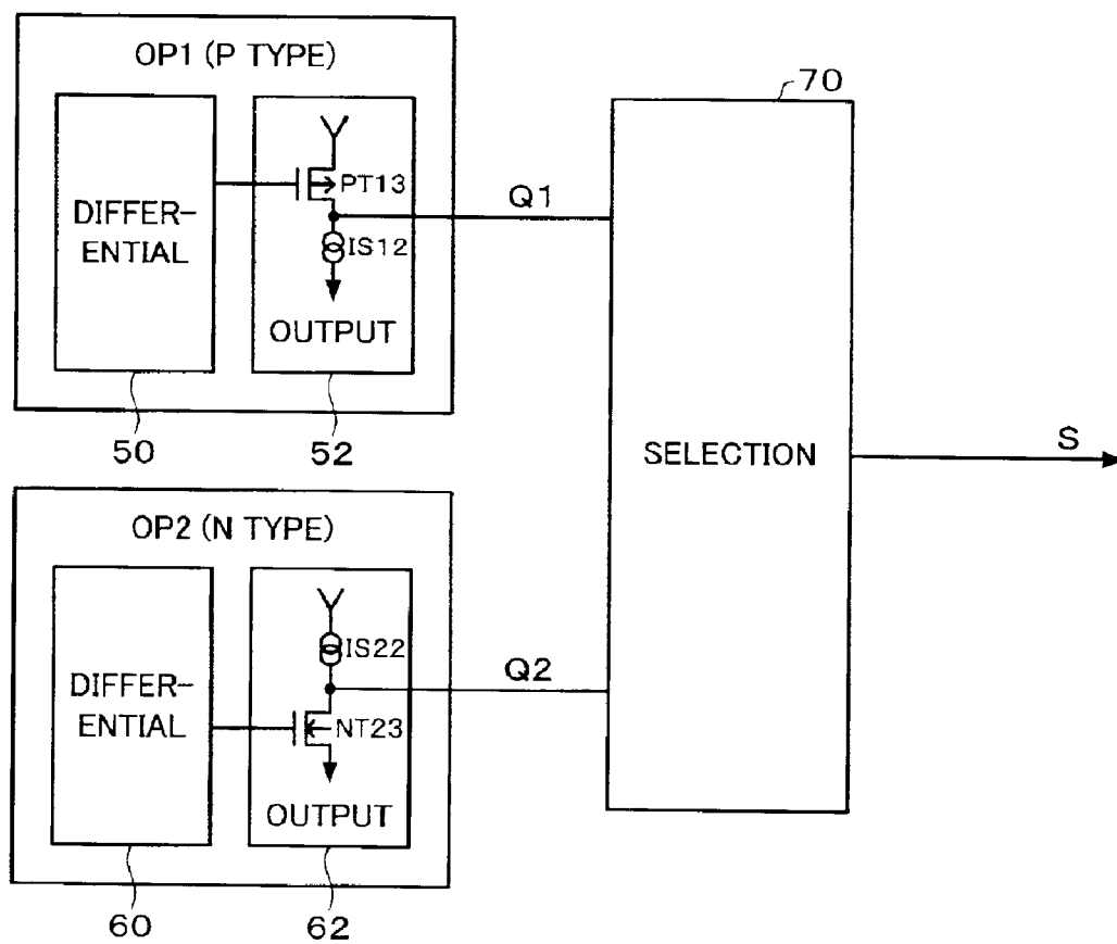
OPERATIONAL AMPLIFIER CIRCUIT
