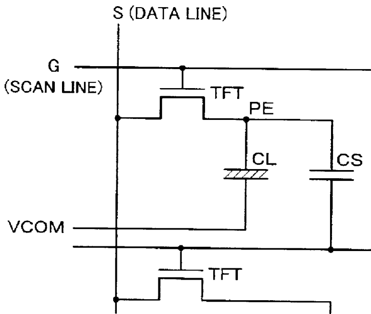
FIG. 12B ADDITIONAL CAPACITANCE METHOD
