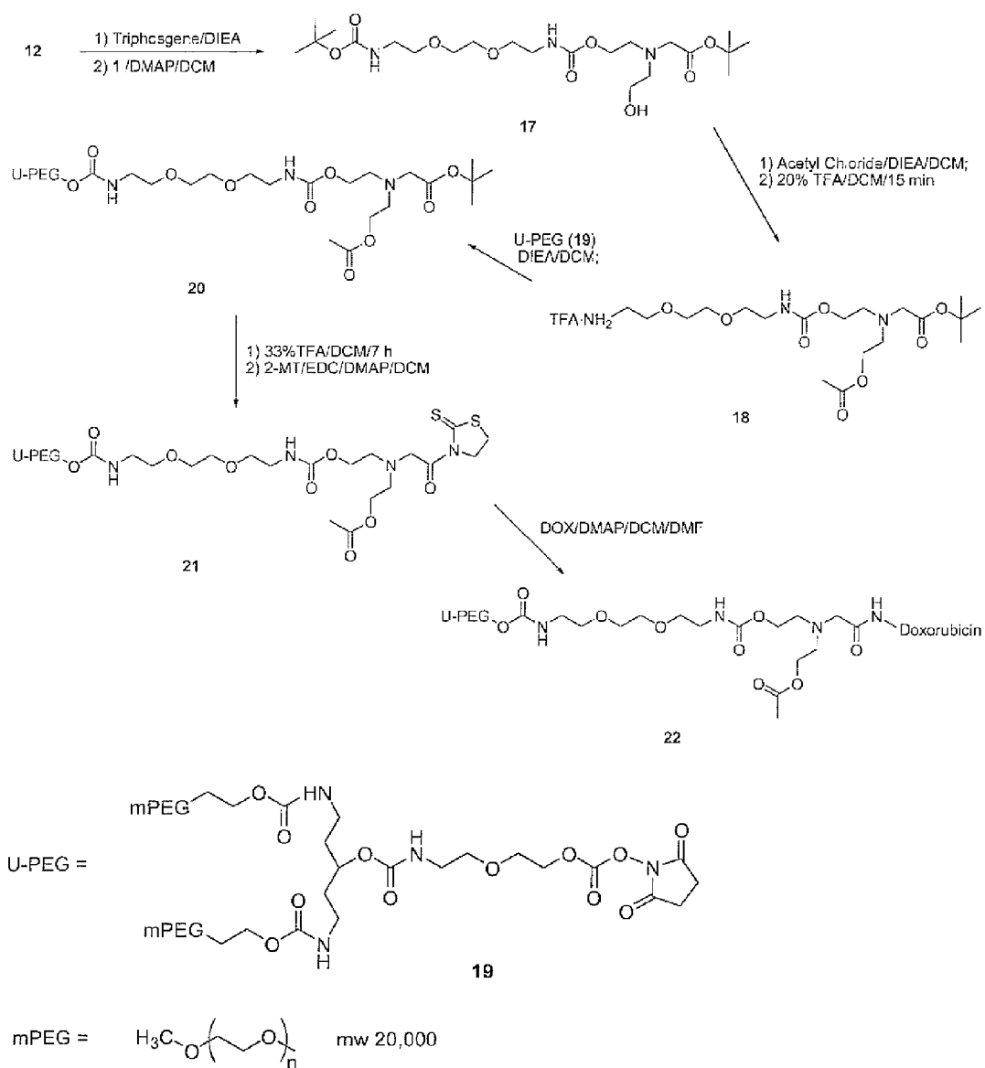
Scheme 4
