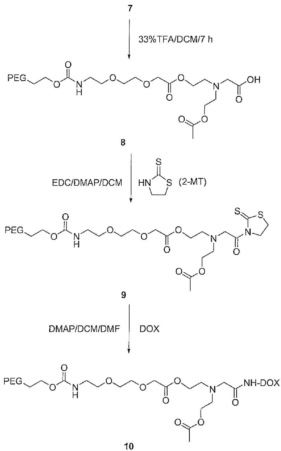
Scheme 2
