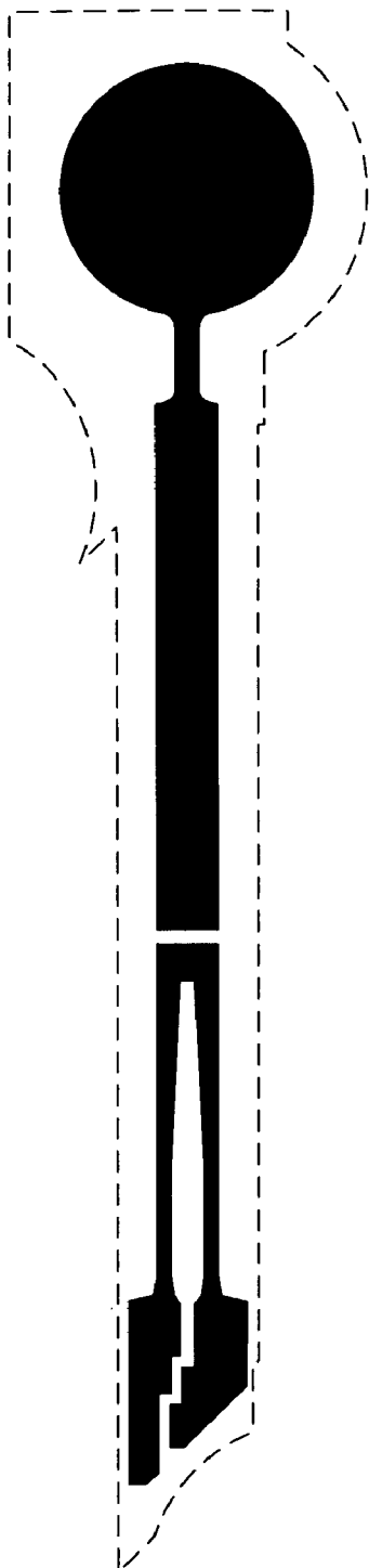
Heater mask
