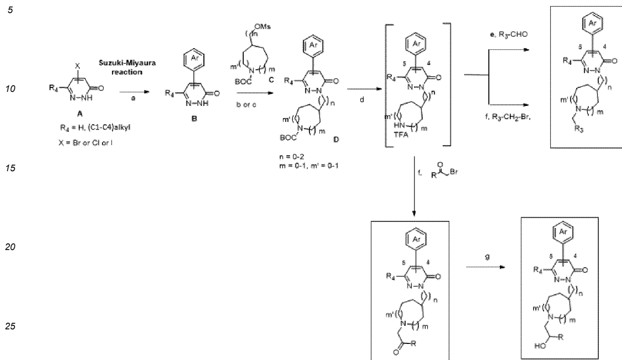
Scheme 1: General synthetic method for the preparation of 2 substituted - N-substituted-piperidin-4-yl -4 or (5) -phenyl pyridazin-3(2H)-one.
