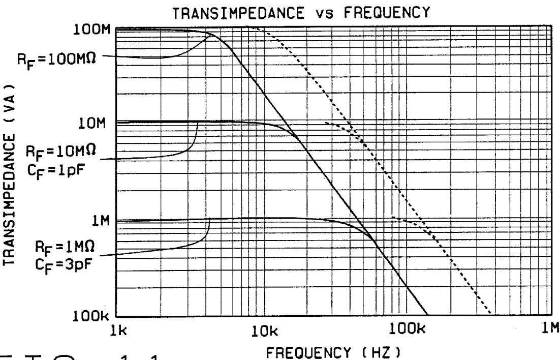
FIG. 11 -----BANDWIDTH WITH BOOTSTRAP BUFFER
