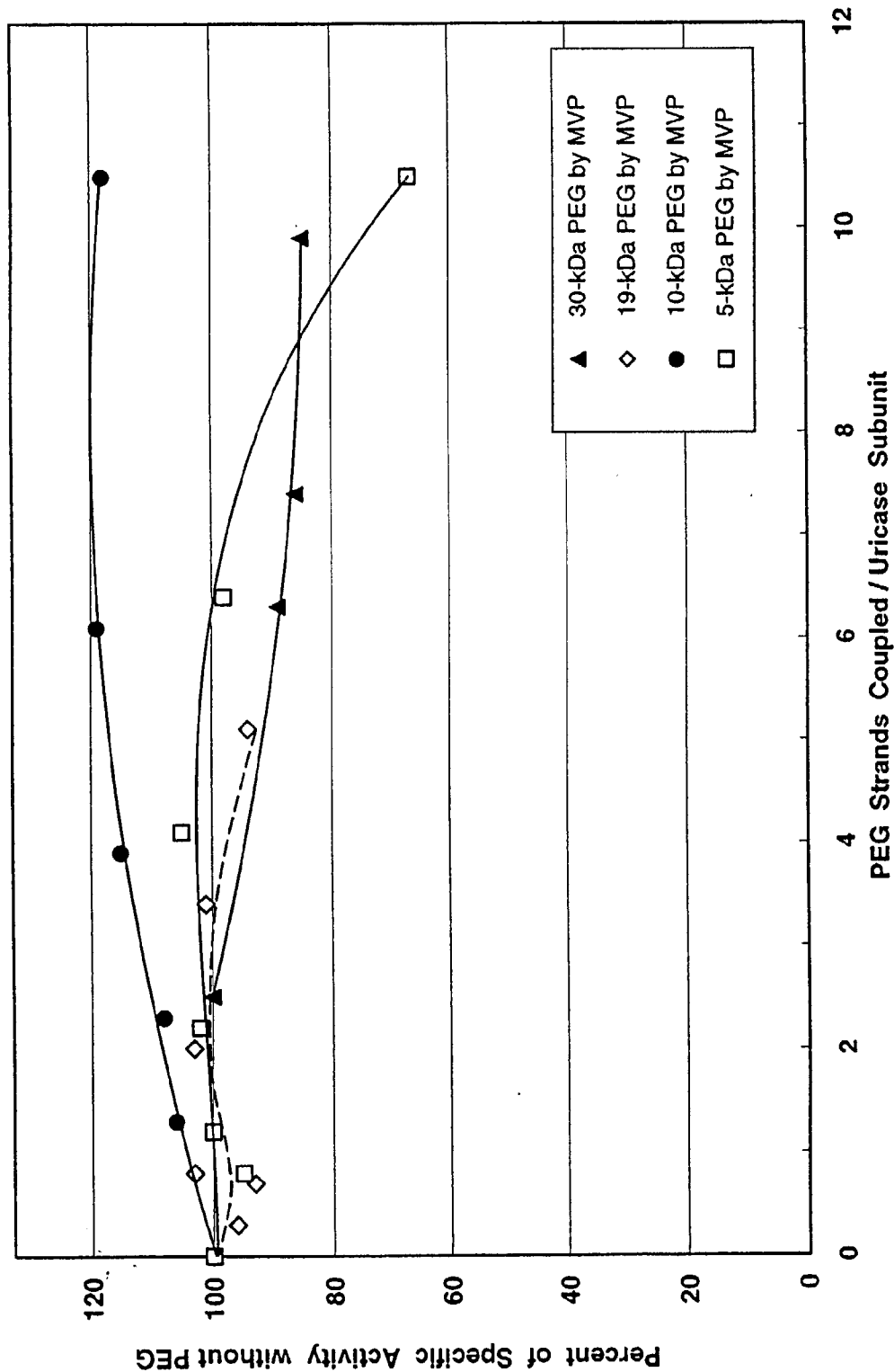
Figure 3A: Retention of Activity by PEGylated PBC Uricase
