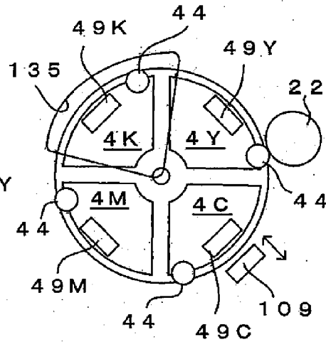
FIG. 5B : DEVELOPMENT POSITION
