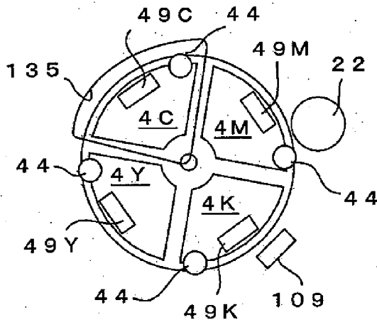
FIG. 5C : MOUNTING/DISMOUNTING POSITION
