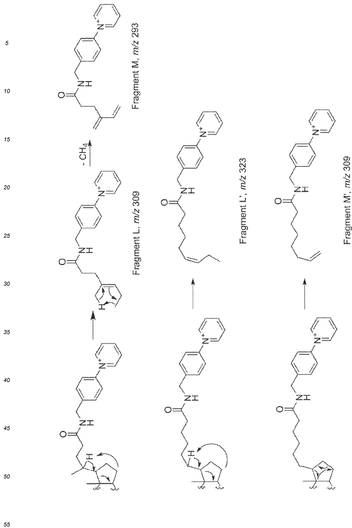
Scheme 3. Proposed fragmentation pathway to fragments L (L')- M (M') in AMPP derivatives of unconjugated bile acids 1 - 7
