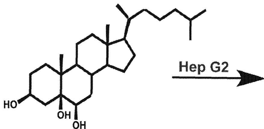
cholestane- 3 \beta ,5 \alpha ,6 \beta -triol
