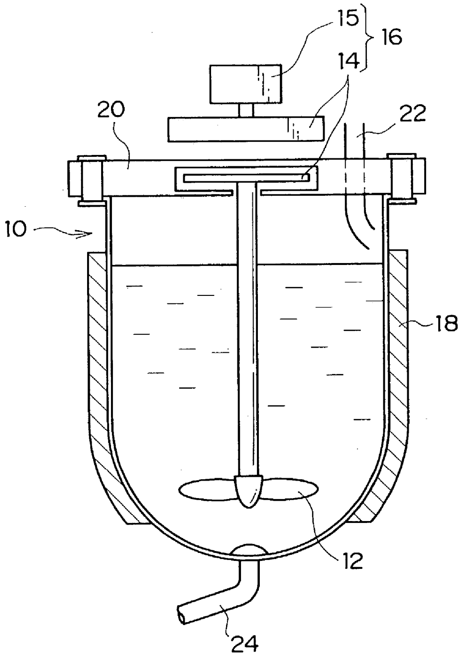
FIG.37 PRIOR ART
