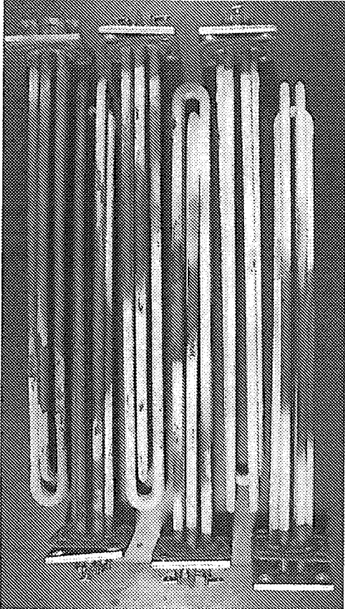
Booster heater with treated water
