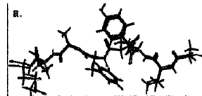
Fig. Comparison of the lowest energy predicted conformation (green) and the experimental structure of a peptide in MHC 20
