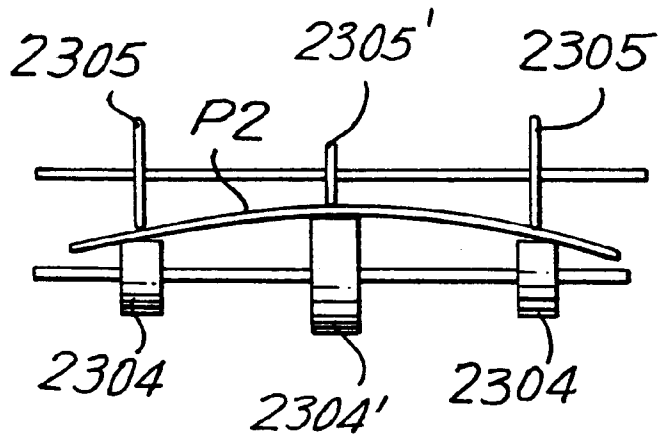
FIG. 67 PRIOR ART
