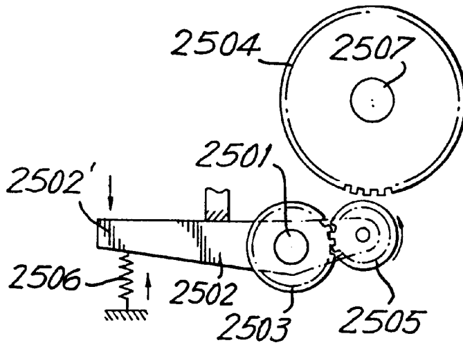
FIG. 60 PRIOR ART
