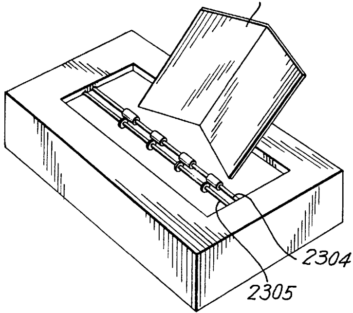
FIG.65 PRIOR ART 2306
