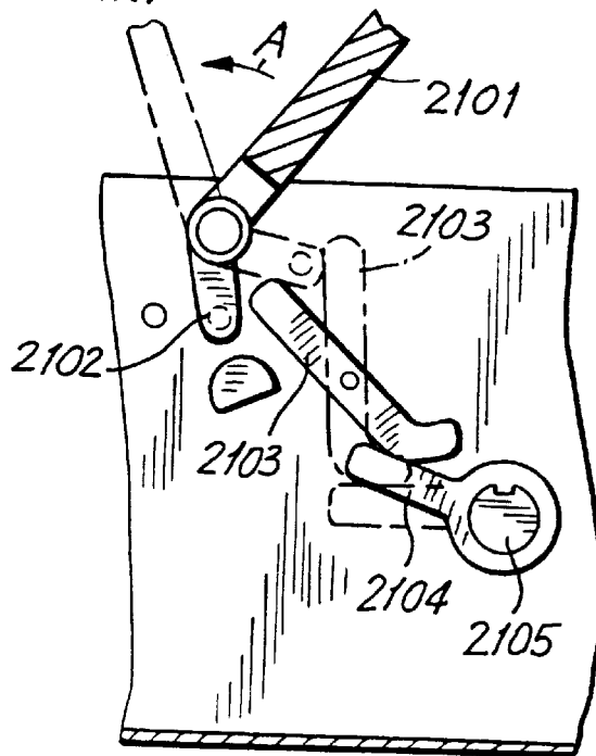
FIG.59 PRIOR ART
