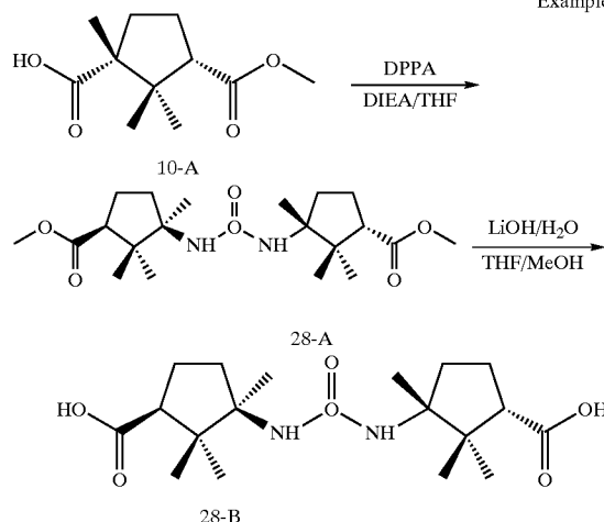
Scheme 28
