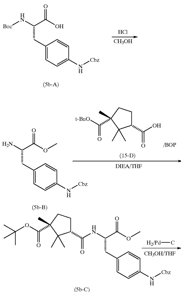
Scheme 5b
