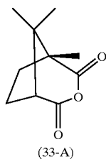
Scheme 33
