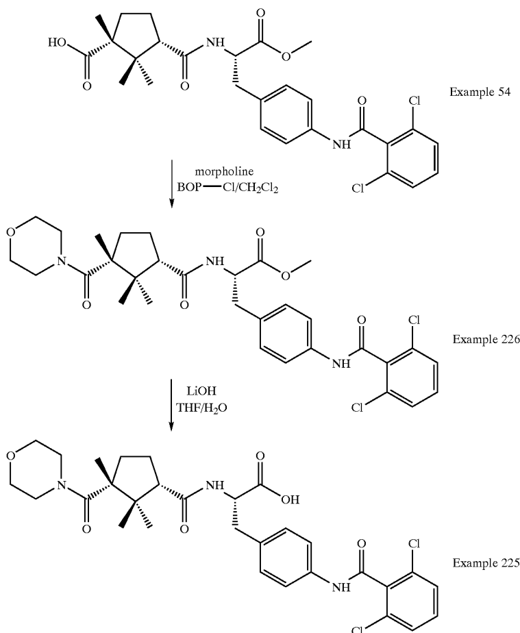
Scheme 27
