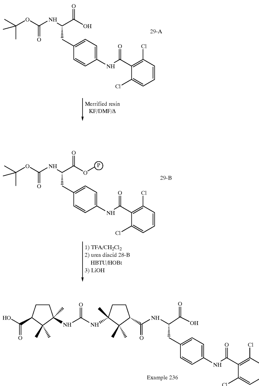
Scheme 29
