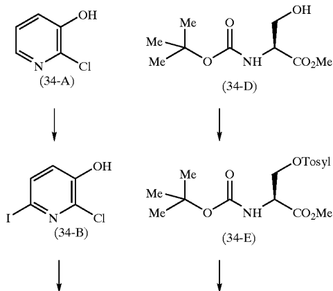
Scheme 34
