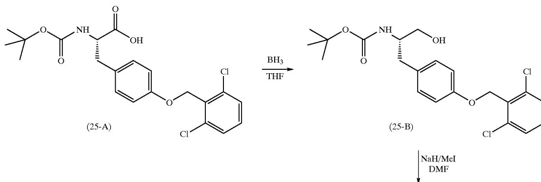
Scheme 25
