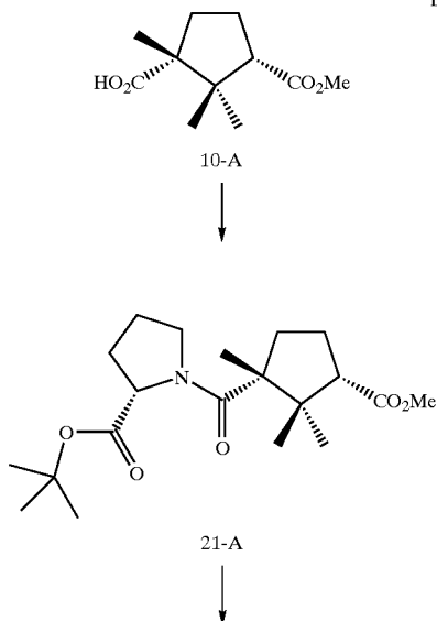
Scheme 21
