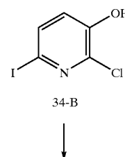
Scheme 39
