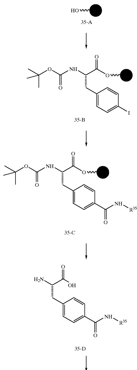
Scheme 35
