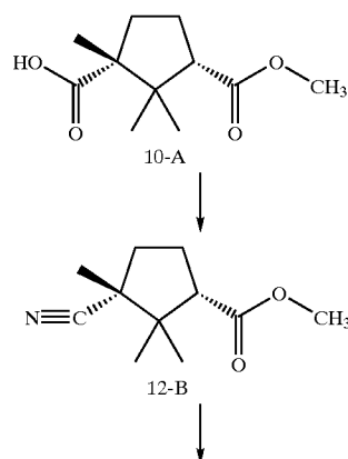
Scheme 12
