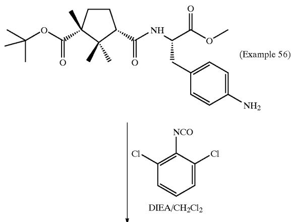
Scheme 26
