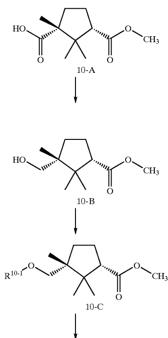
Scheme 10
