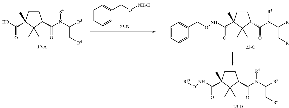
Scheme 23
