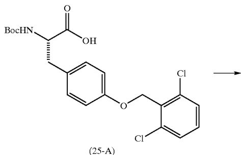
Scheme 30
