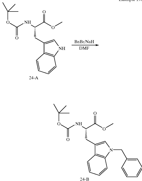
Scheme 24
