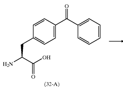
Scheme 32
