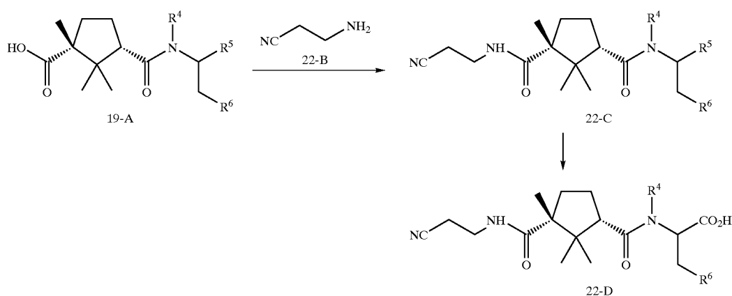
Scheme 22
