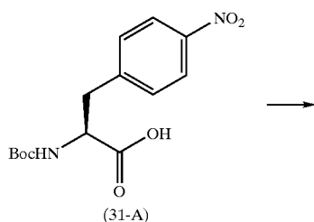
Scheme 31
