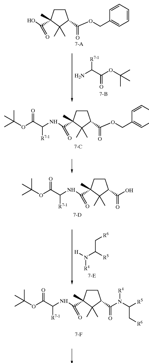
Scheme 7
