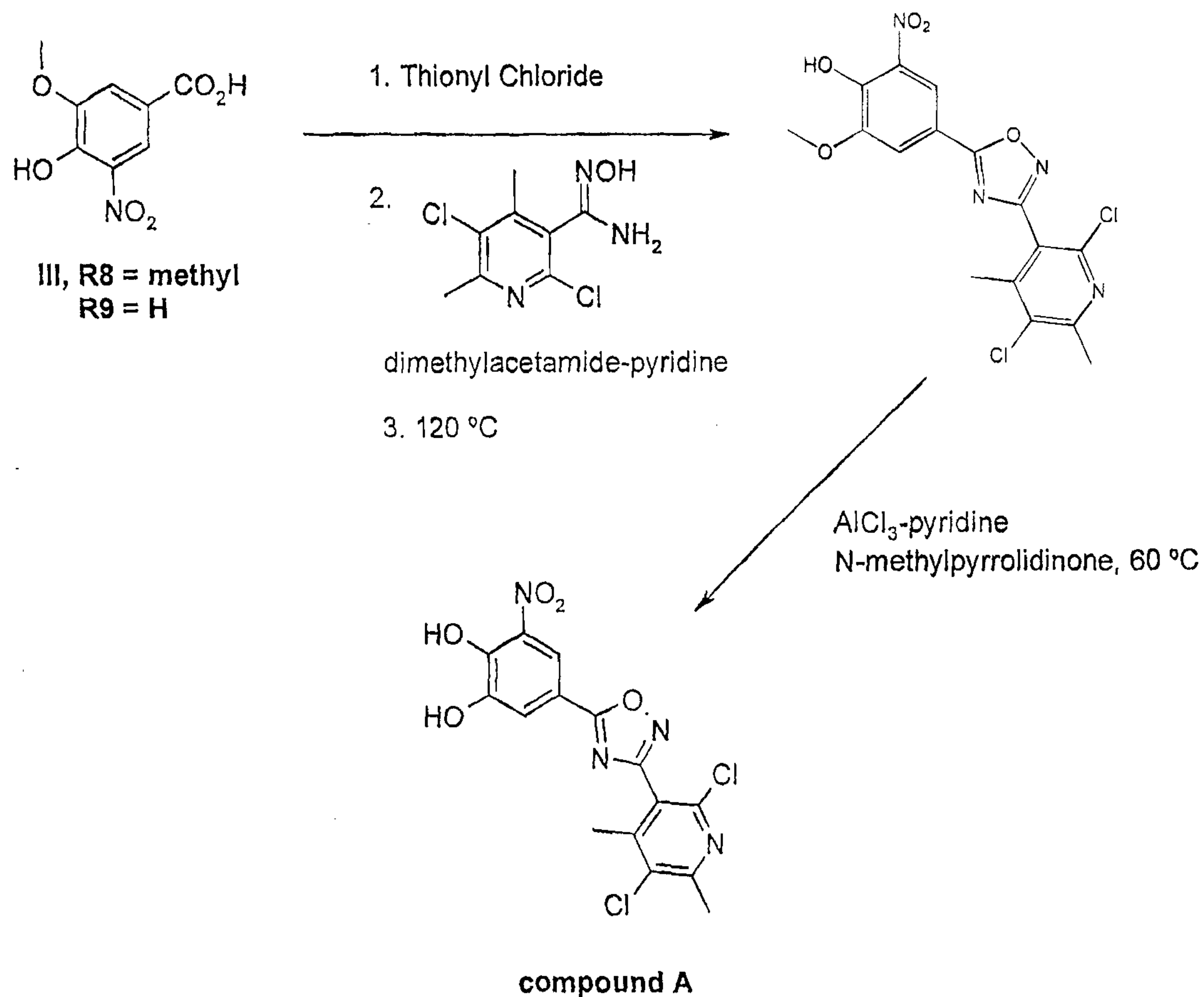
Scheme 3. Preparation of compound A
