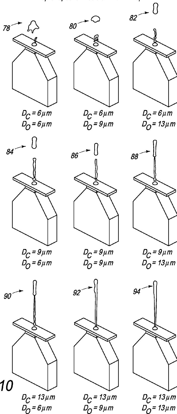
Drop Shapes for Resistor Width = 20\mu m
