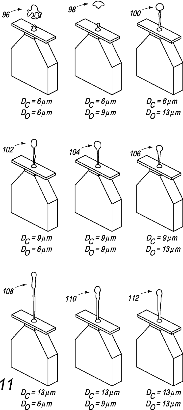
Drop Shapes for Resistor Width = 32\mu\text{m}
