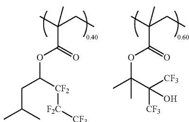
Water-repellent polymer 2 M w = 8,300 M w /M n = 1.84
