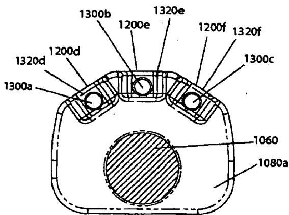
Fig. 11 (Section A-A of Fig. 7 )
