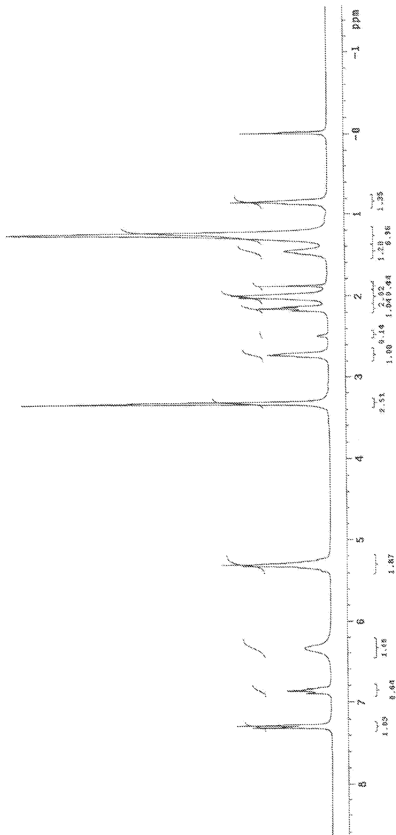
CLX-SYN-GI77C-5-1A, DMSO-d6
