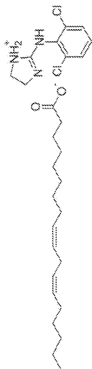
CLX-SYN-GI77C-5-1A, DMSO-d6
