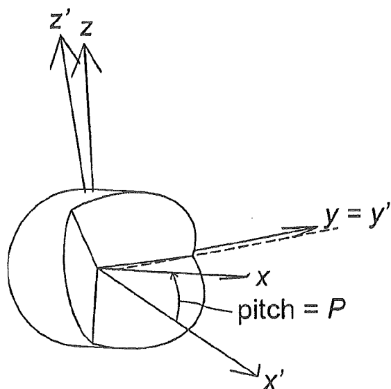
PERSPECTIVE VIEW Figure 9a
