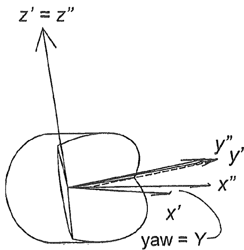
PERSPECTIVE VIEW Figure 10a
