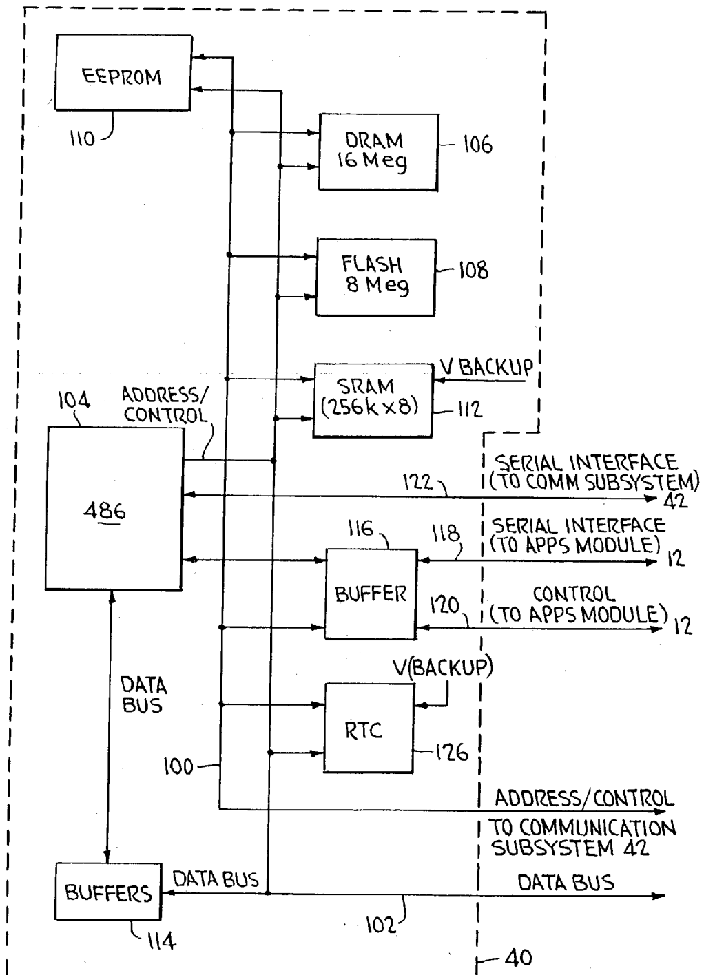
FIG. 3 PROCESSOR SUBSYSTEM
