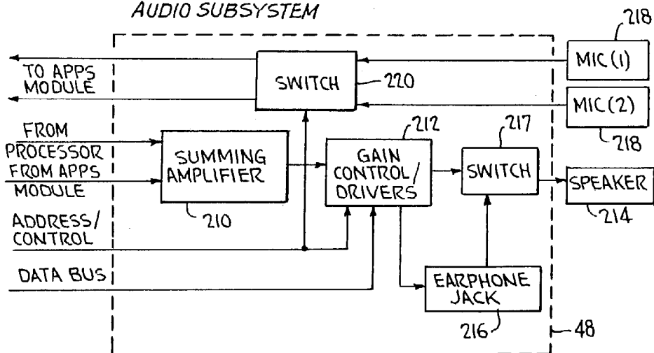
FIG. 7 AUDIO SUBSYSTEM
