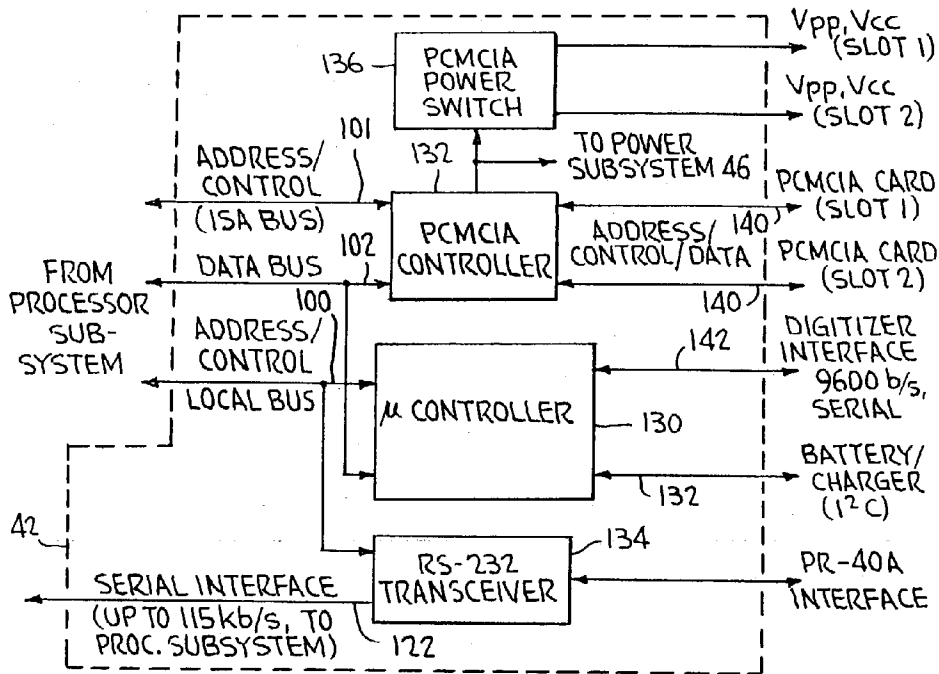
FIG. 4 COMMUNICATION SUBSYSTEM
