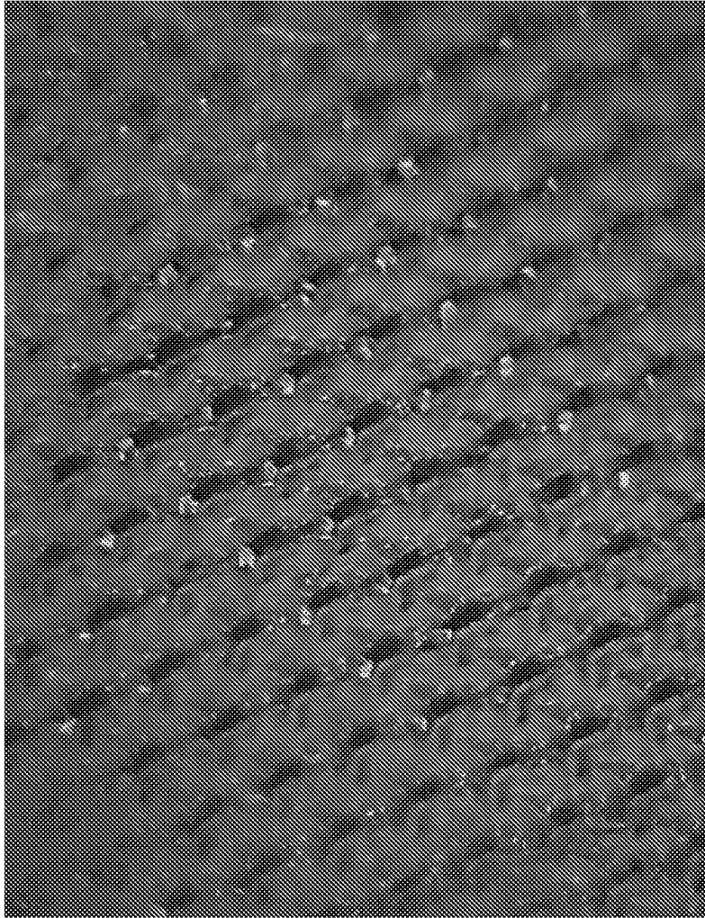
Example section from non-capped 3D printed microfluidic device, 20 um pillars x 200 um tall, offset at 10 um 80 um spacing – printed in 4x exposure without moving stage.
