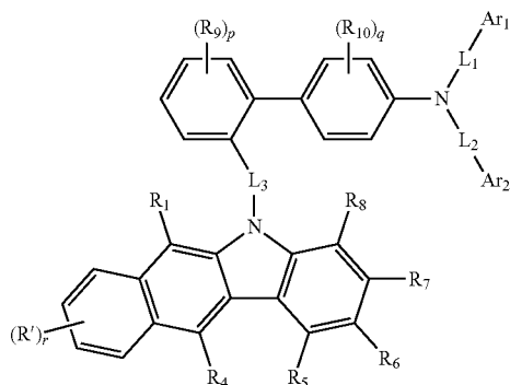
[Chemical Formula 3]
