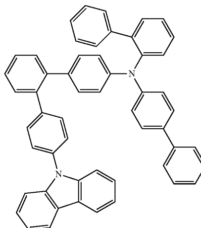
[Compound 1-10]
