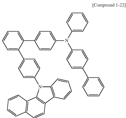
[Compound 1-22]
