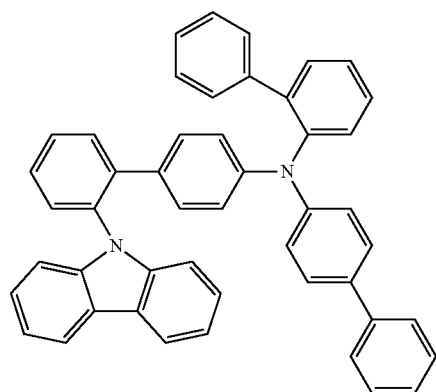
[Compound 1-20]
