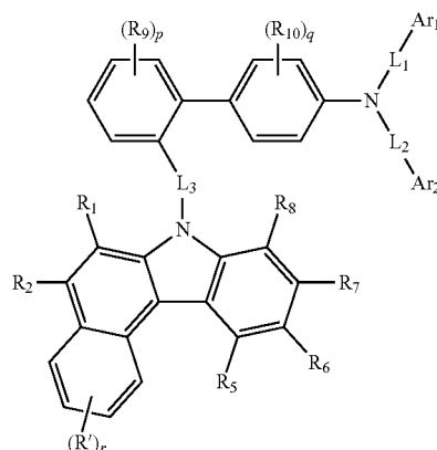
[Chemical Formula 4]
