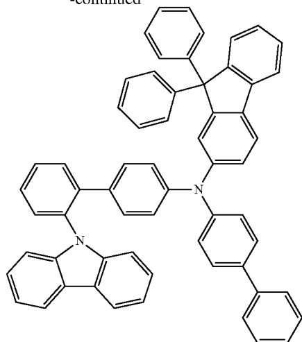
[Compound 1-6]
