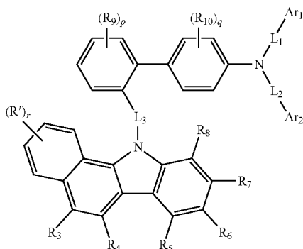
[Chemical Formula 3]
