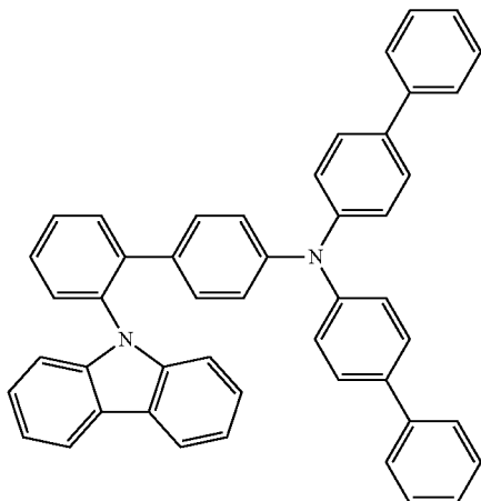
[Compound 1-1]
