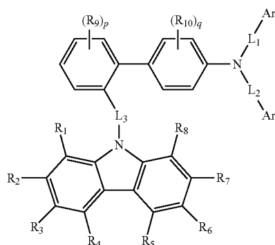
[Chemical Formula 1]
