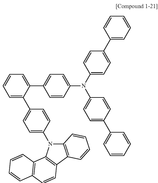
[Compound 1-21]
