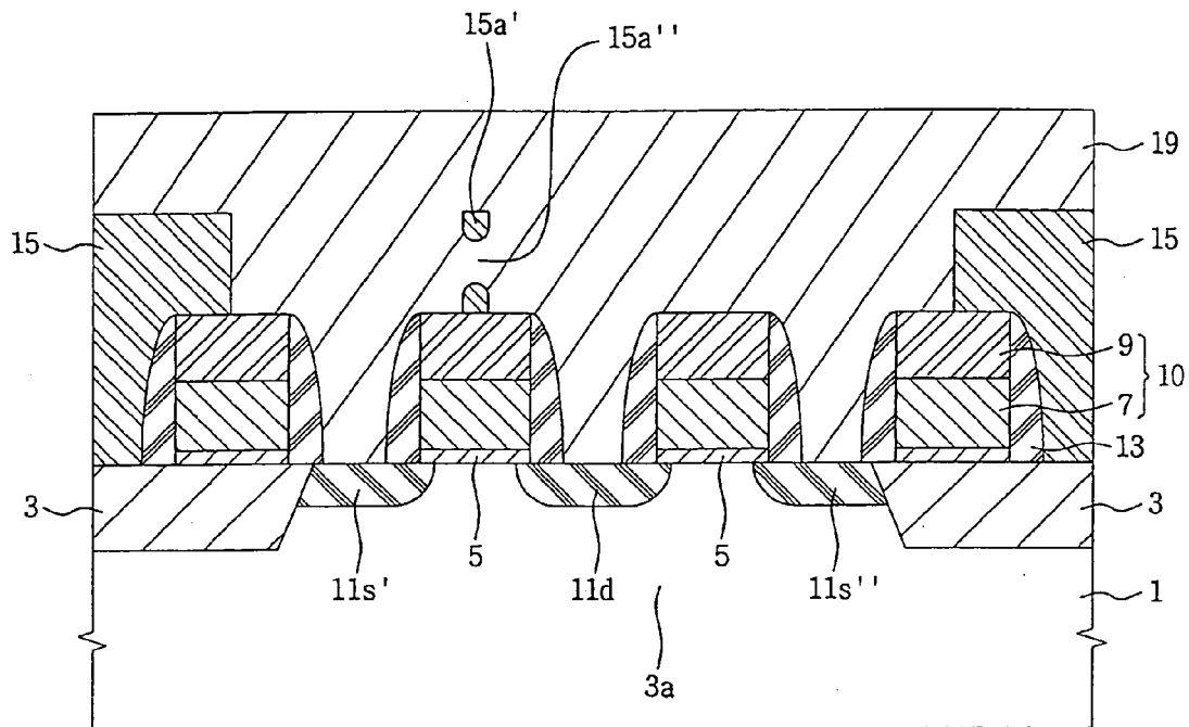
FIG. 3 (CONVENTIONAL ART)
