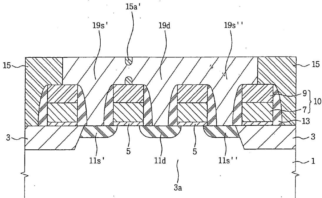
FIG. 4 (CONVENTIONAL ART)
