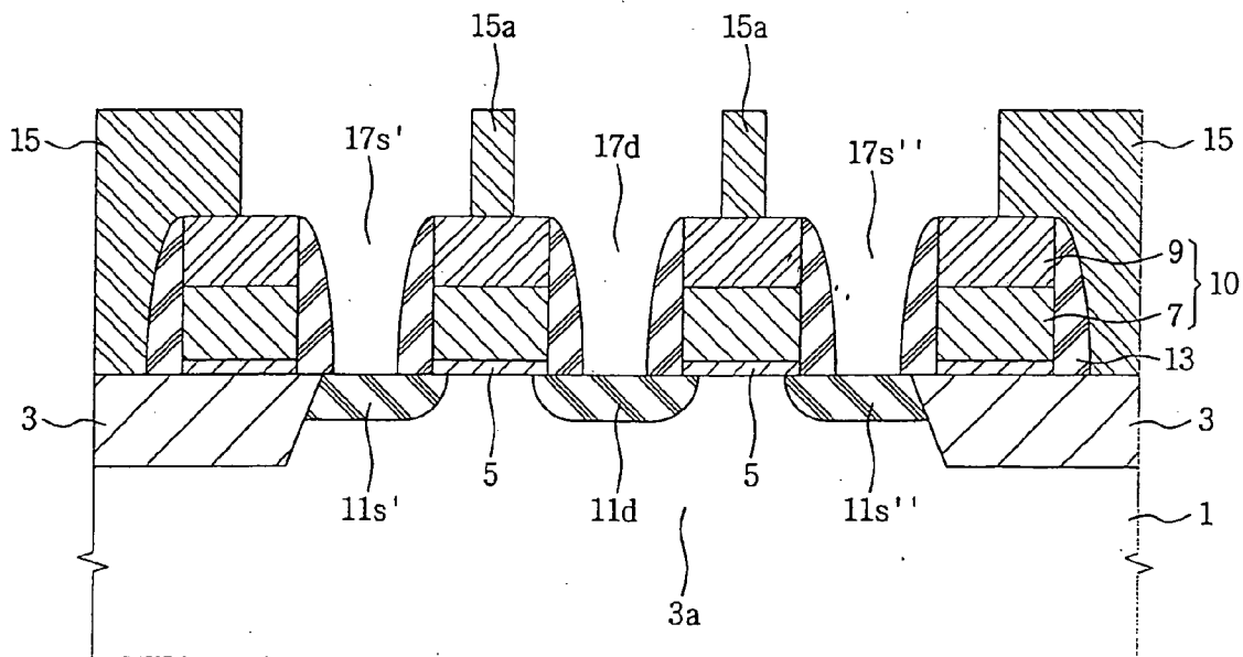
FIG. 2 (CONVENTIONAL ART)
