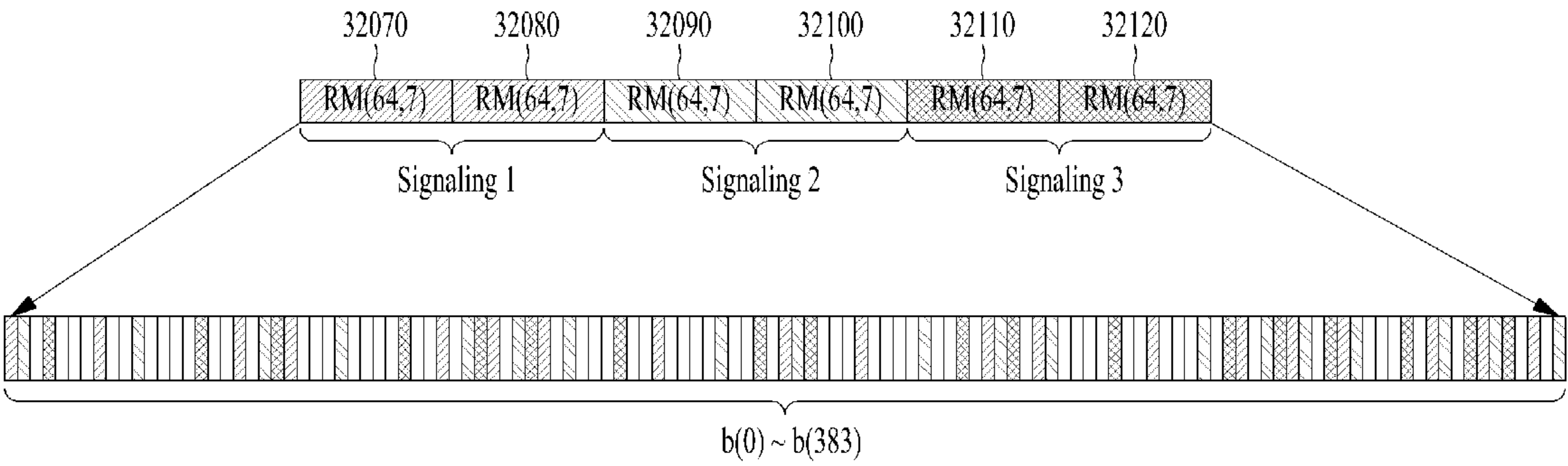
(b) 21bit signaling with 64bit Reed Muller FEC block case
