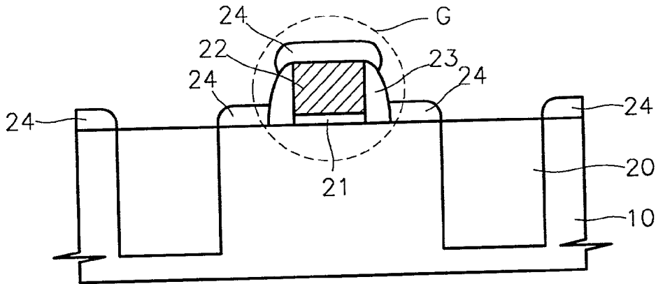
FIG. 4 (PRIOR ART)
