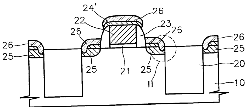
FIG. 5 (PRIOR ART)
