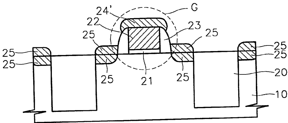
FIG. 4 (PRIOR ART)
