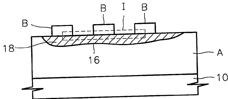
FIG. 2C (PRIOR ART)
