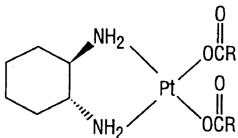
DACH Platinum(II) Complex
