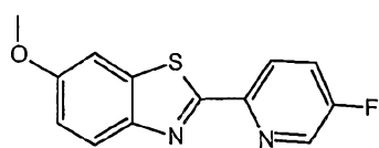
2-(5-fluoropyridin-2-yl)-6-methoxy-1,3-benzothiazole
