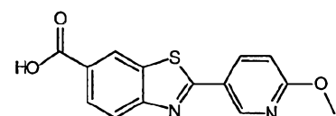
2-(6-Methoxypyridin-3-yl)-1,3-benzothiazole-6-carboxylic Acid
