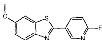
2-(6-Fluoropyridin-3-yl)-6-methoxy-1,3-benzothiazole
