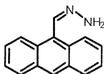
Intermediate \gamma
