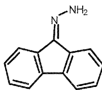
Intermediate \beta
