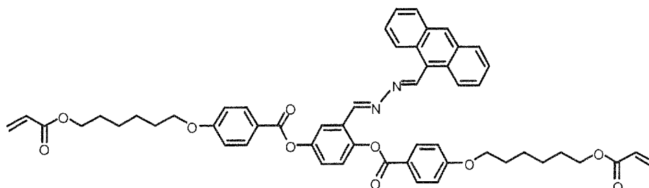
Compound 2r
