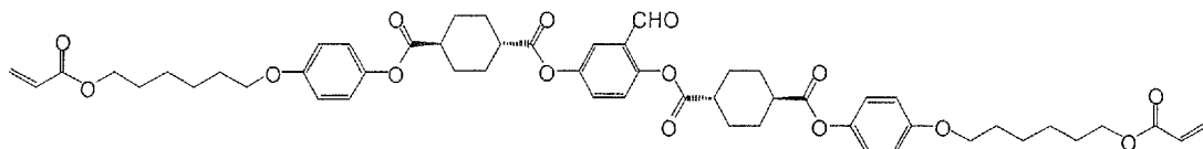
Intermediate B
