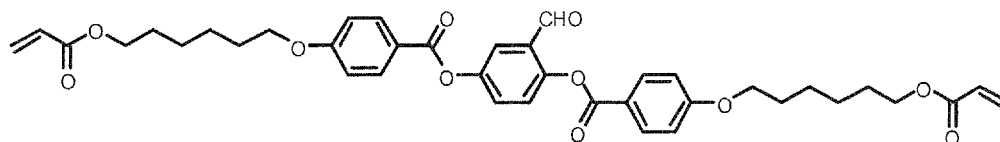
Intermediate \alpha
