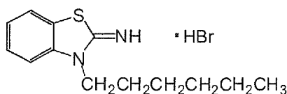
Intermediate C
