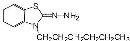
Intermediate D
