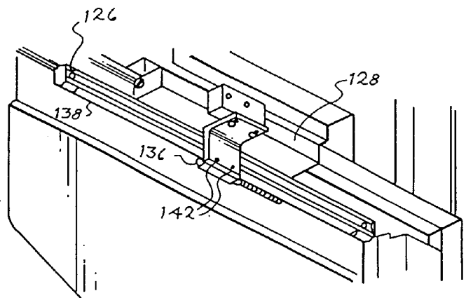
Fig. 8 (PRIOR ART)
