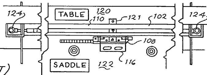
Fig. 5 (PRIOR ART)
