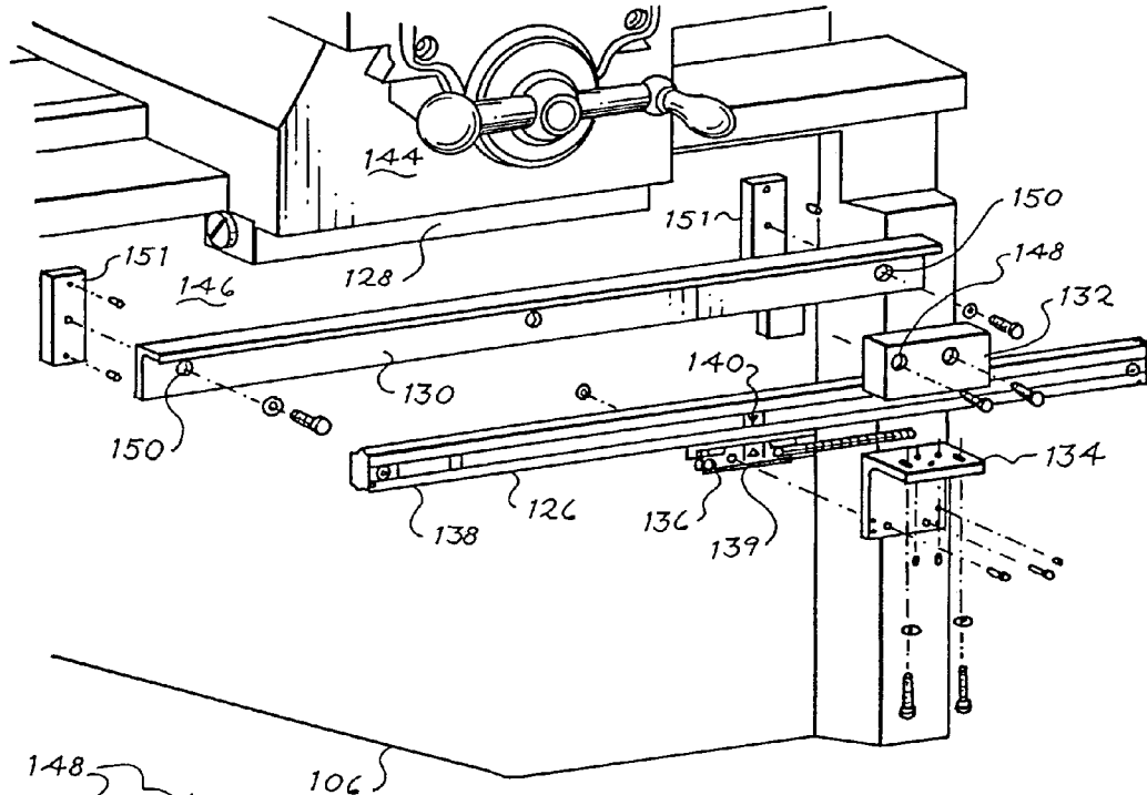
Fig. 6 (PRIOR ART)
