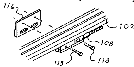
Fig. 5 (PRIOR ART)
