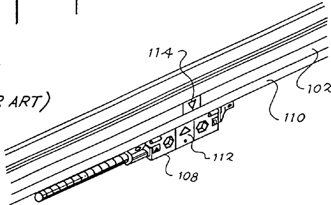
Fig. 3 (PRIOR ART)
