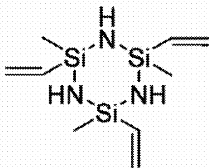
1,3,5-trivinyl-1,3,5-trimethylcyclotrisilazane (V 3 N 3 , CAS# 5505-72-6)
