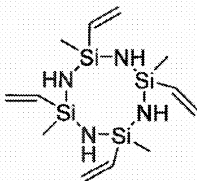
1,3,5,7-tetravinyl-1,3,5,7-tetramethylcyclotetrasilazane (V 4 N 4 , CAS# 5162-63-0)
