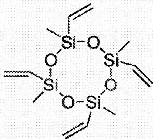
1,3,5,7-tetravinyl-1,3,5,7-tetramethylcyclotetrasiloxane (V 4 D 4 , CAS# 2554-06-5)
