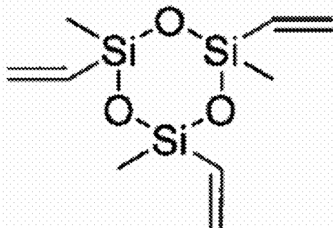
1,3,5-trivinyl-1,3,5-trimethylcyclotrisiloxane (V 3 D 3 , CAS# 3901-77-7)
