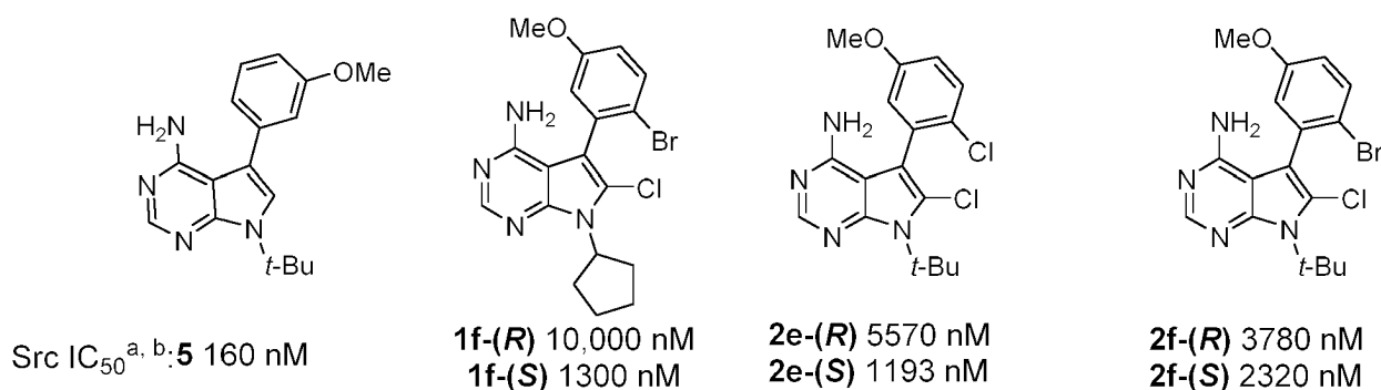
Scheme 3. Differential Src kinase inhibitory activities between atropisomers.
