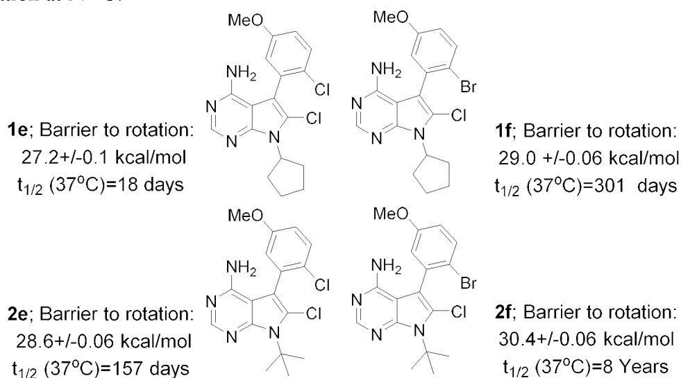
Scheme 2. Experimentally measured barriers to rotation, and extrapolated t_{1/2} to racemization at 37 °C.
