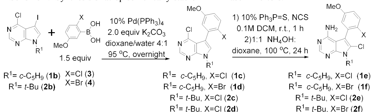
Scheme 1. Synthesis of atropisomerically stable PPY kinase inhibitors.
