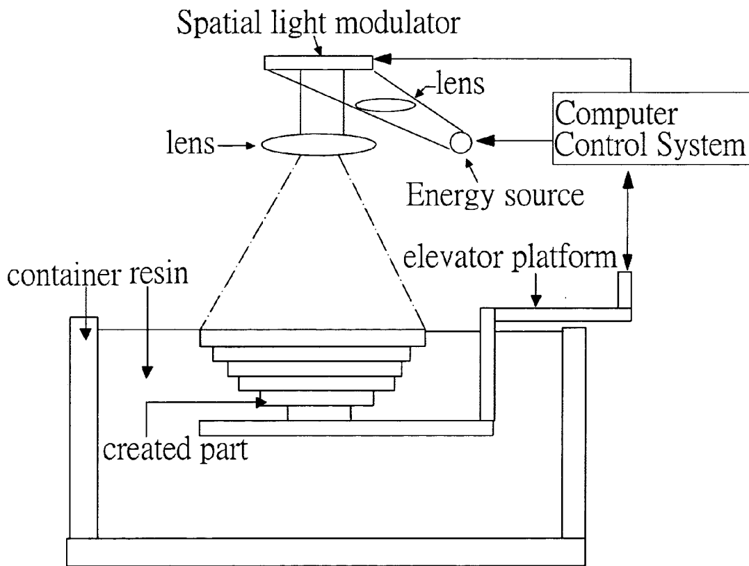
FIG 6 PRIOR ART
