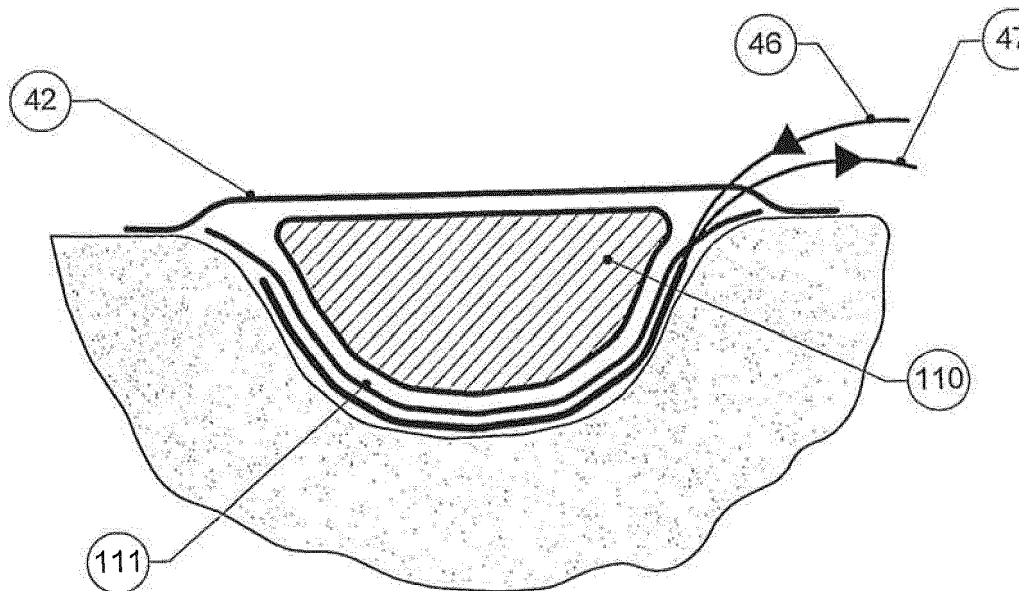
Section Through X -X
