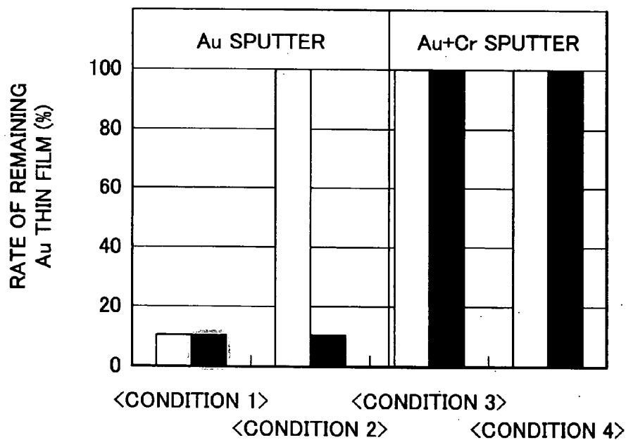
ADHESION OF Au THIN FILM TYPE SEPARATOR
