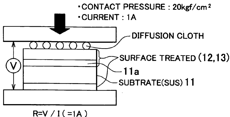
CONTACT RESISTANCE TEST METHOD
