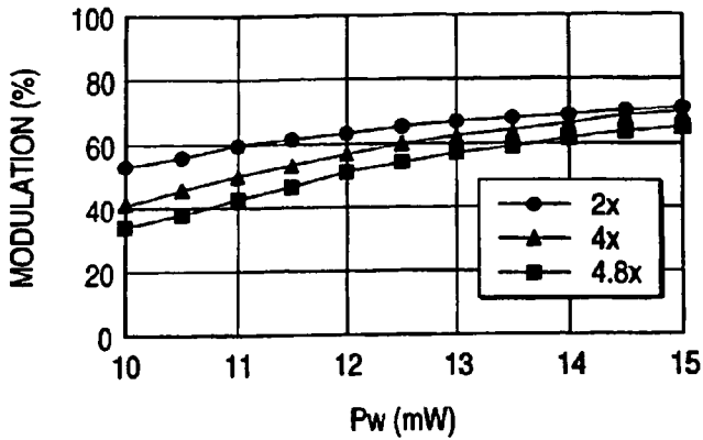
RECORDING POWER DEPENDENCY OF MODULATION
