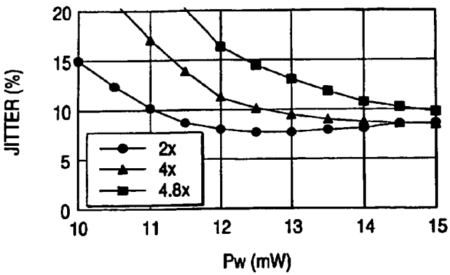
RECORDING POWER DEPENDENCY OF EDGE-TO-CLOCK JITTER
