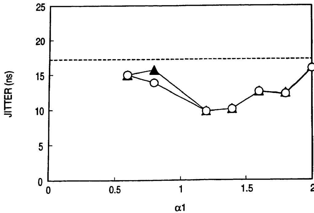
MARK AND SPACE JITTER
