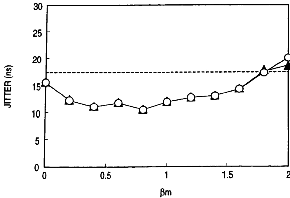
MARK AND SPACE JITTER
