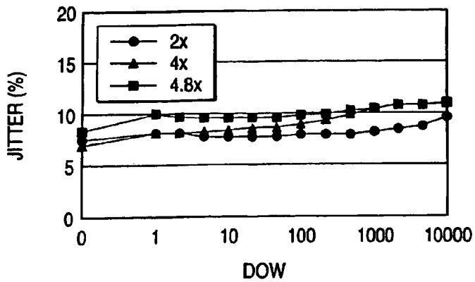
OVERWRITE CYCLE DEPENDENCY OF EDGE-TO-CLOCK JITTER
