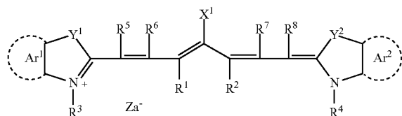
Formula (a)
