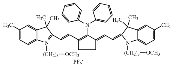
Infrared absorber (1)
