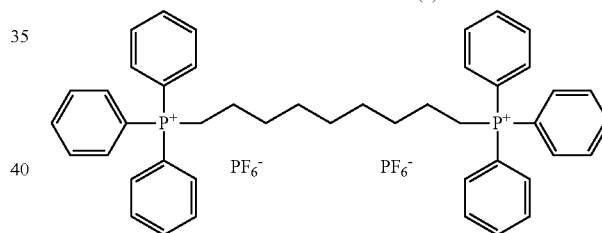
Phosphonium compound (1)
