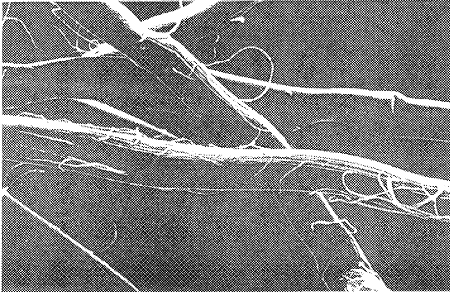
Abraded Commercial Fiber 1 - 1000X
