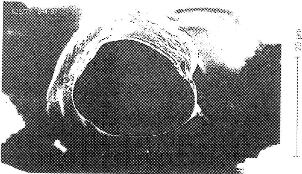
Centrifugally Spun Fiber End - 2,000X
