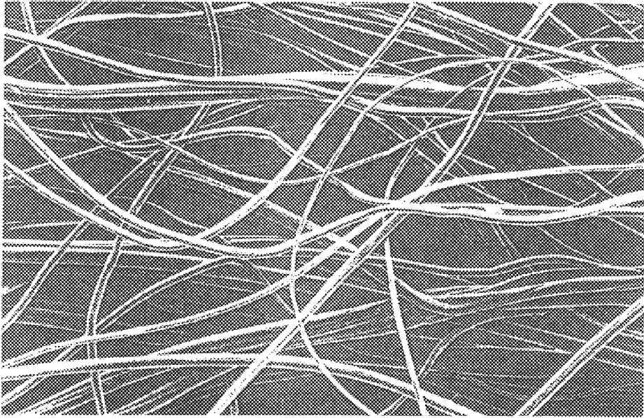
Centrifugally Spun Fiber - 200X
