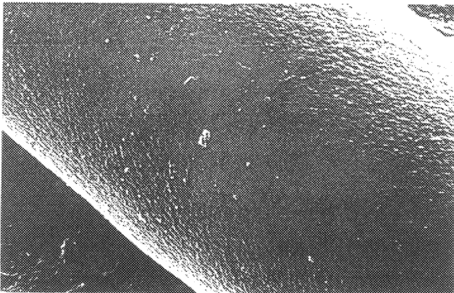
Centrifugally Spun Fiber - 10,000X
