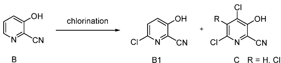
Scheme I
